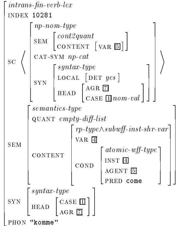
Figure 1: The simplified feature structure for the German verb komme (to come).
