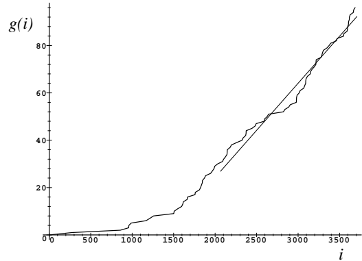
Figure 2: Estimation of the current OOV word probability for word category CITY.
