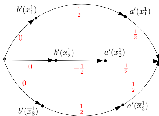
Figure 3.5: Gadget for C_1 in \phi = (x_1 \vee x_2 \vee \bar{x}_3) \wedge (x_1 \vee \bar{x}_2 \vee x_3) \wedge (\bar{x}_1 \vee x_2 \vee x_3)
