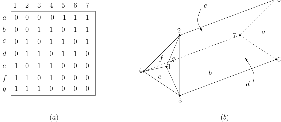
Figure 8.2: A 3-dimensional self-dual indecomposable polytope and its incidence matrix.
