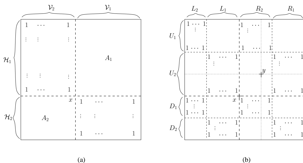
Figure 8.1: The incidence matrix C = \mathcal{I}(P_1 * P_2) before and after applying the permutations \sigma and \rho . In (b), the two dotted lines, crossing at y , indicate the partition of C^T resulting from the original partition of C . In particular, the upper-right corner above y contains the matrix A_2^T , while the lower-left corner contains A_1^T .
