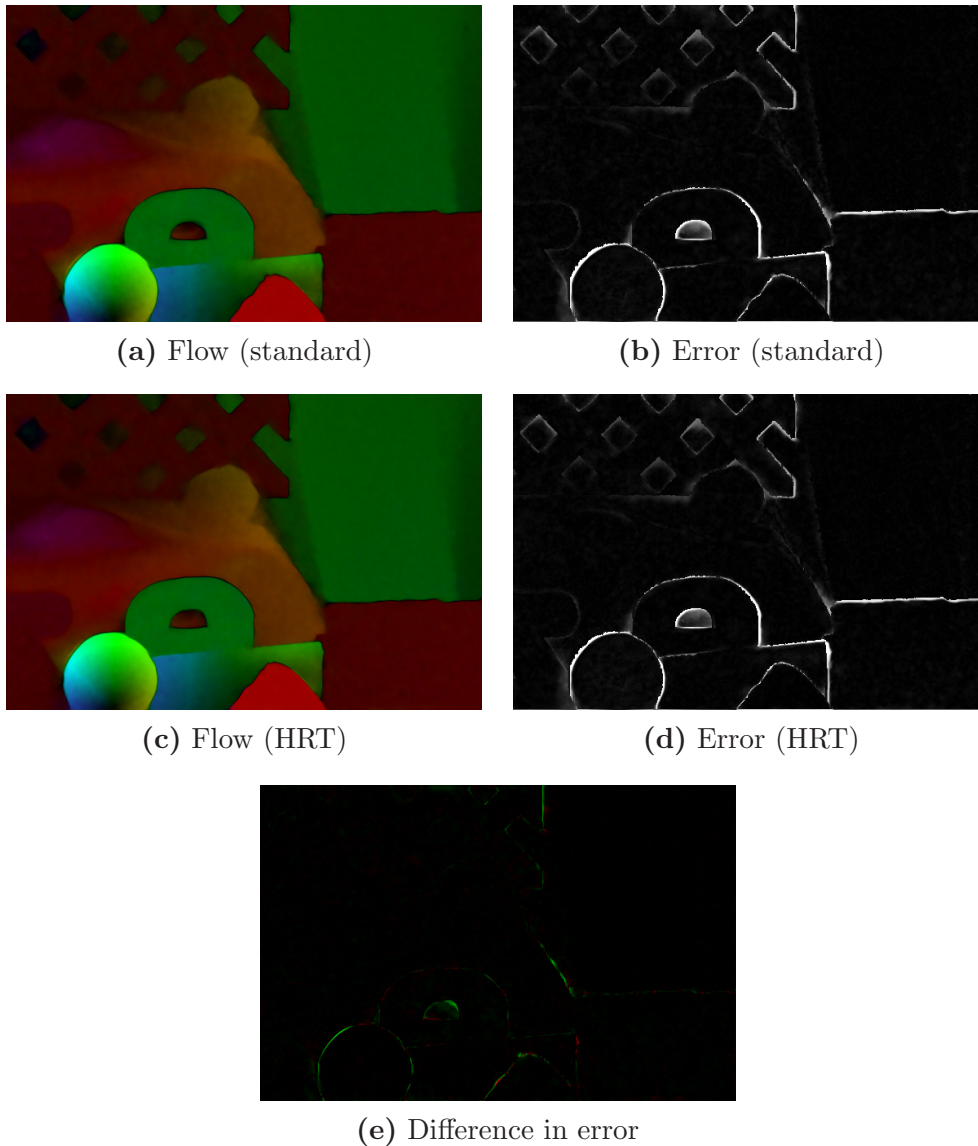
Figure 5.7: Comparison of a “standard”, central derivative approximation of second order to our proposed HRT scheme (on the Rubberhale sequence). Top row, from left to right: (a) Flow field obtained with standard derivative approximation. (b) Corresponding error map visualising the AAE (brighter pixels mark higher errors). Middle row, from left to right: (c) Flow field obtained with our proposed HRT scheme. (d) Corresponding error map. Bottom row: (e) Difference of the error maps in (b) and (d). Green marks improvements, red impairments of our HRT scheme compared to the standard scheme.
