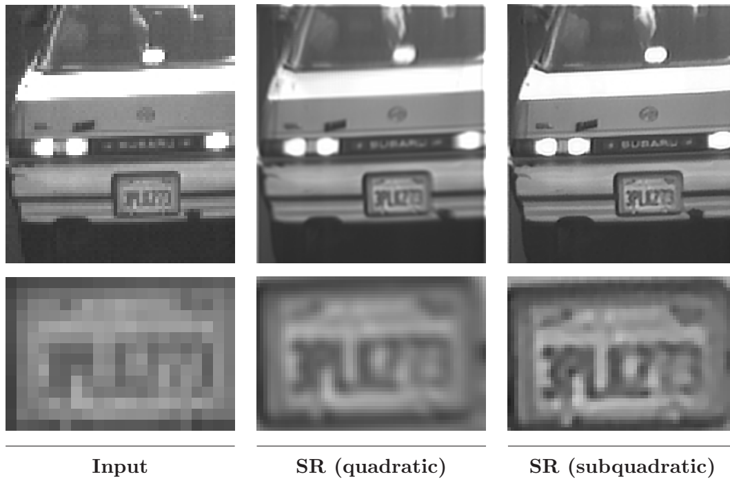
Figure 6.15: Super-resolution example. First row, from left to right: (a) One of the input images (64 images, 72 \times 121 pixels, taken from http://users.soe.ucsc.edu/~milanfar/software/sr-datasets.html ). (b) Super-resolution result using a quadratic data term and a homogeneous smoothness term ( \vartheta = 1.0 ). The used zoom factor was z = 3 . (c) Same using a L_1 data term and a TV smoothness term ( \vartheta = 0.7 ). Second row, from left to right: (d)–(f) Zooms in (a)–(c).
