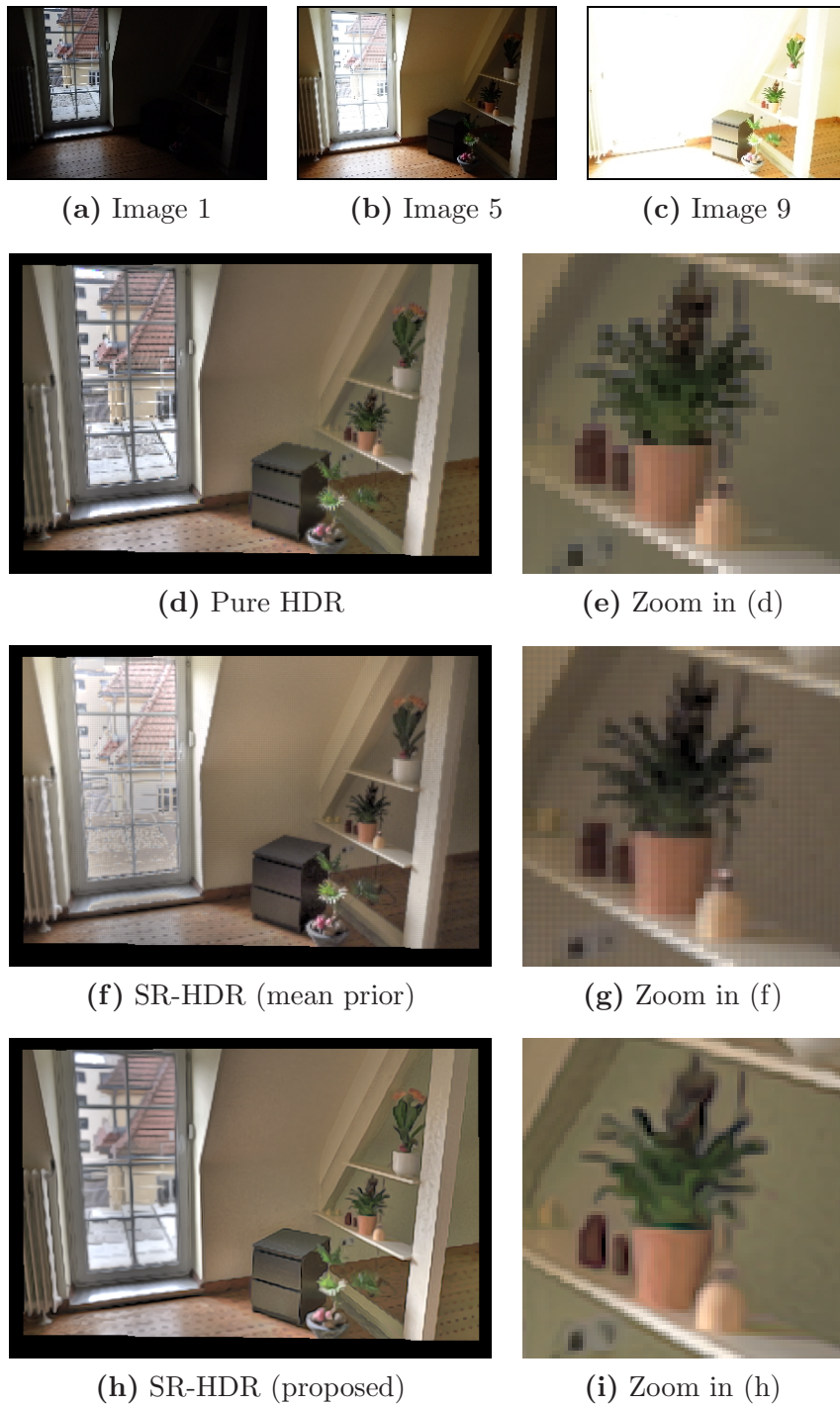
Figure 6.16: Joint SR-HDR reconstruction on a real world exposure series. First row, from left to right: (a) – (c) Images 1, 5 and 9. Second row, from left to right: (d) Upsampled HDR reconstruction. (e) Zoom in (d). Third row, from left to right: (f) SR-HDR result of [CPK09, GG06] (quadratic data term, mean prior, \vartheta=5.0, \tau=0.1 , 25 iterations). (g) Zoom in (f). Fourth row, from left to right: (h) Result of proposed method ( \vartheta=0.3, s=8, \rho_1=0.4, \rho_2=0.2, \tau=0.5 , 1000 iterations). (i) Zoom in (h).
