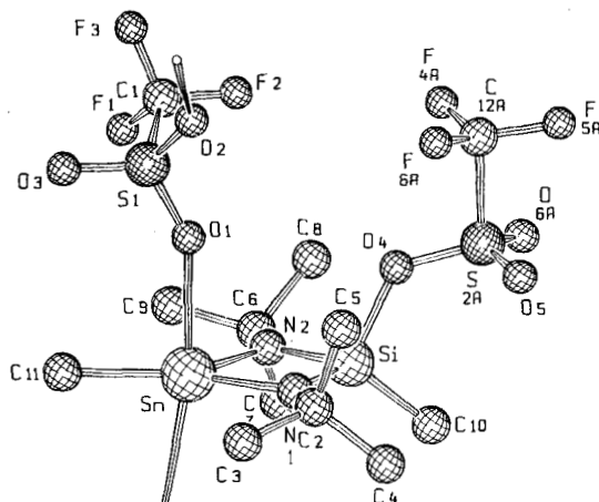
FIGURE 1 The structure and atom numbering of (F_3C-SO_3)(Me)Sn(NtBu)_2Si(Me)(O_3S-CF_3) ( 2 ).
