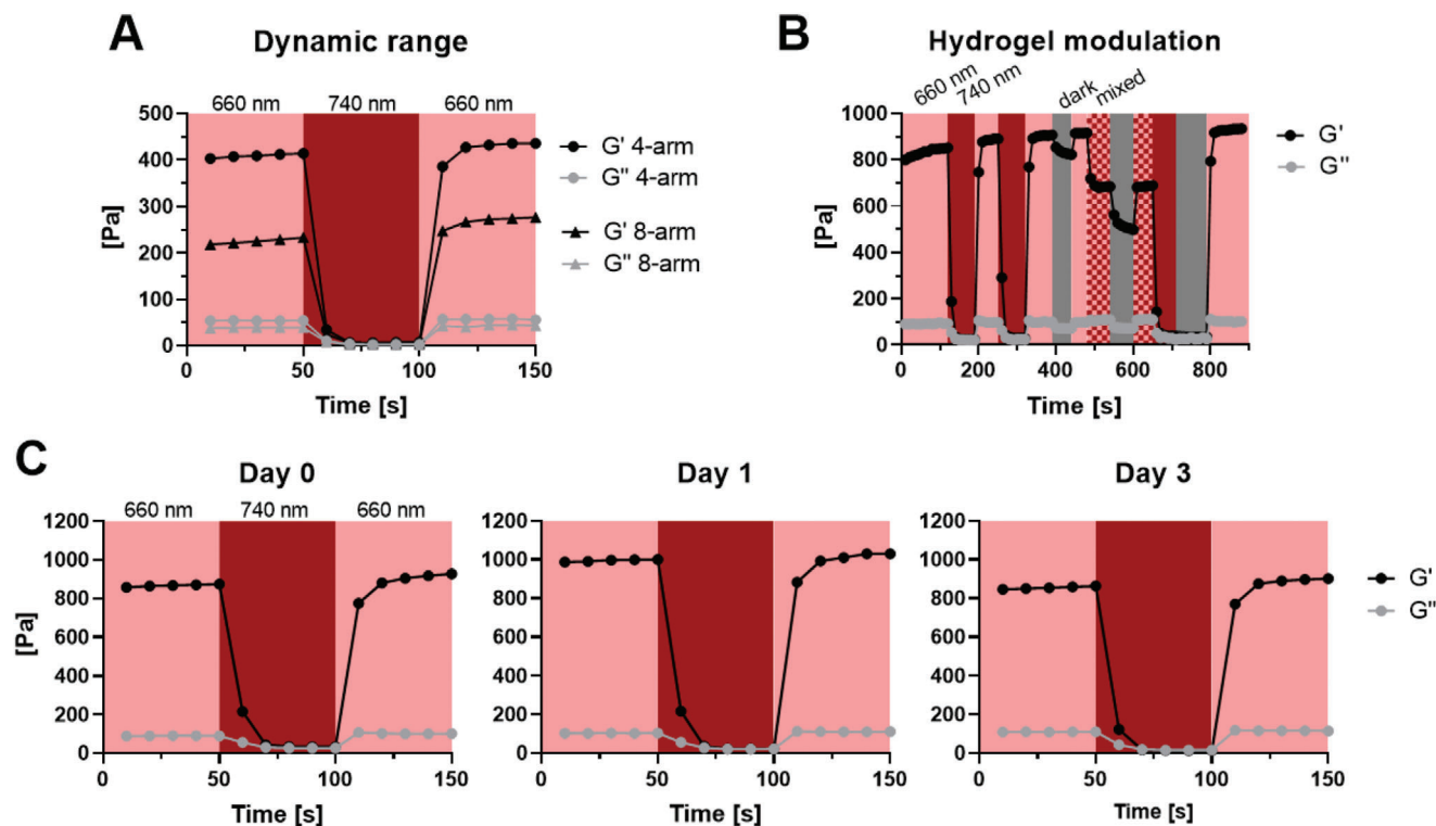
Figure 3. Characterization of light-dependent hydrogel mechanics. PEG-PhyB and PEG-PIF6 were mixed under 740 nm illumination and storage ( G' ) and loss ( G'' ) modulus of PEG-PhyB- and PEG-PIF6-based materials were recorded by small amplitude oscillatory shear rheology over time in response to different illumination conditions: 660 nm: light red; 740 nm: dark red; 660 and 740 nm light: checked; no light: grey. A) 4-arm or 8-arm PEG-PhyB was mixed with 8-arm PEG-PIF6 (final coupled PhyB concentration: 50 mg ml -1 ) under 740 nm illumination, illuminated with 660 nm for gelation and the light-dependent mechanical properties were recorded. B) A hydrogel consisting of 4-arm PEG-PhyB and 8-arm PEG-PIF6 (final coupled PhyB concentration: 85 mg ml -1 ) was prepared and analyzed as described in (A). C) Dynamic range and functionality of the hydrogel variant from (B) was tested at 0, 24, and 72 h after initial hydrogel preparation.
