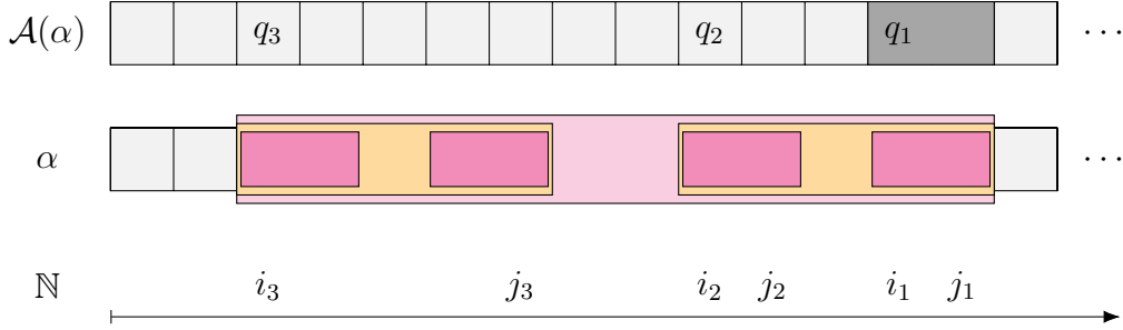
Figure 3.1: Constructing (i_2, j_2) and (i_3, j_3) from u := \alpha[i_1, j_1] . \blacksquare , \blacksquare , \blacksquare , \blacksquare represent the finite words u, v_1, v_2, v_3 , respectively. Observe that v_1 is a prefix of v_2 , which itself is a prefix of v_3 .
