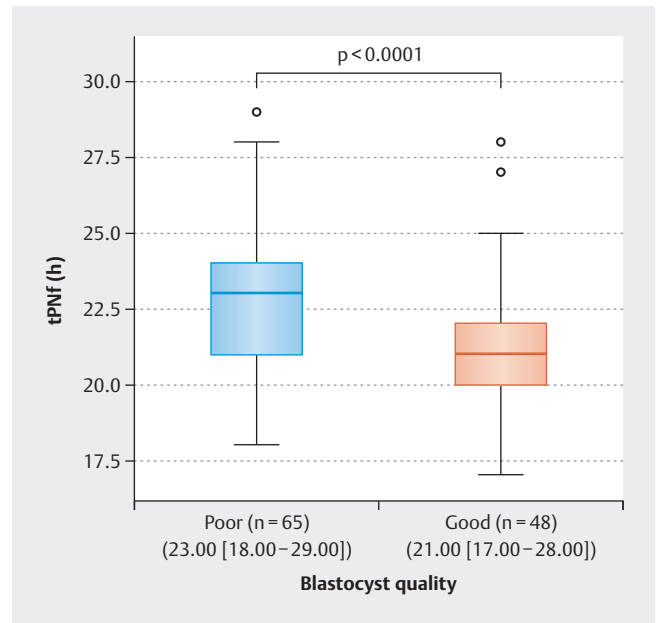
► Fig. 4 The difference in pronuclear fading time between poor (n = 65) and good (n = 48) blastocyst quality groups (23.00 h [18.00–29.00] vs 21.00 h [17.00–28.00], retrospectively; p < 0.0001 ). Results are presented as median (range). p is calculated using the Mann–Whitney U test.
