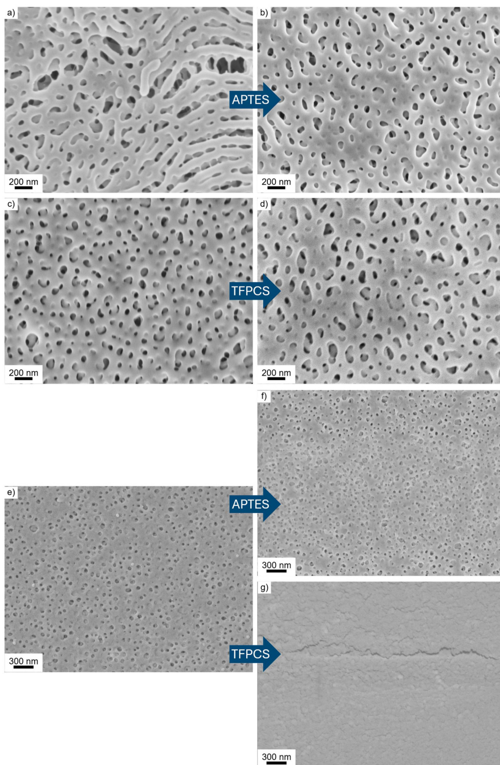
Fig. 5 Membranes based on the linear BCP are shown before post-modification (a, c) and after post-modification with APTES (b) and TFPCS (d). Membranes based on star-shaped BCPs ( M3 ) before post-modification (e) and after post-modification with APTES (f) and TFPCS (g).
